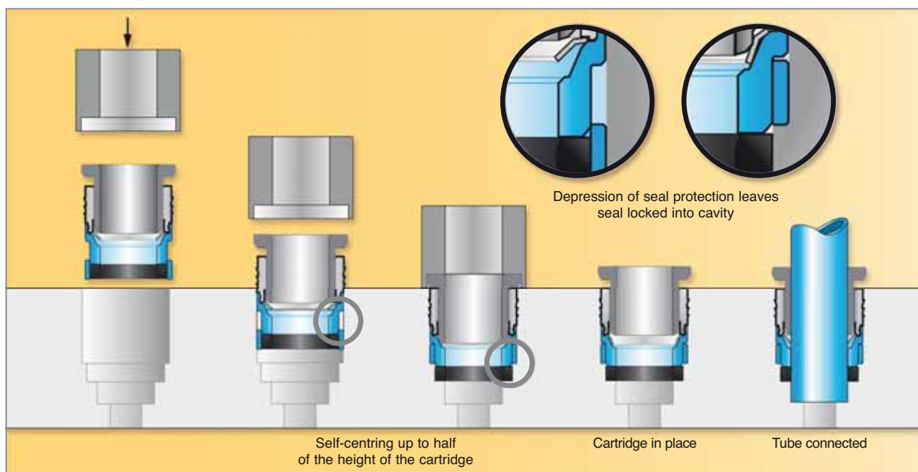
Assembly tool
