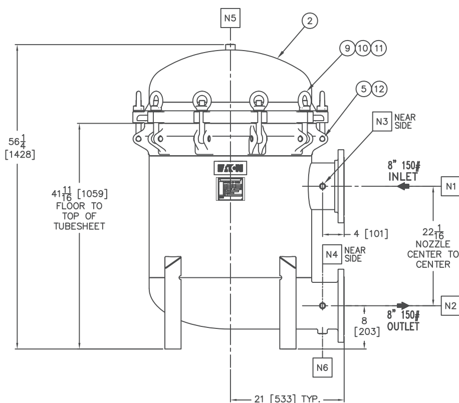
NOZZLE SCHEDULE
