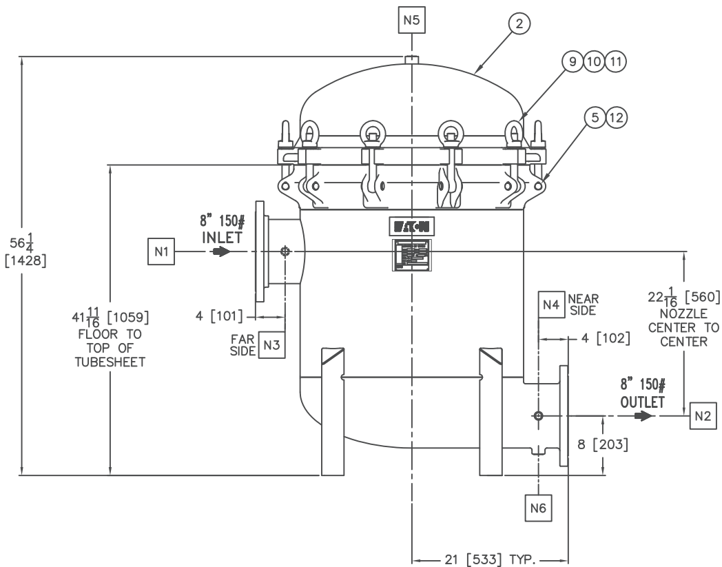
NOZZLE SCHEDULE
