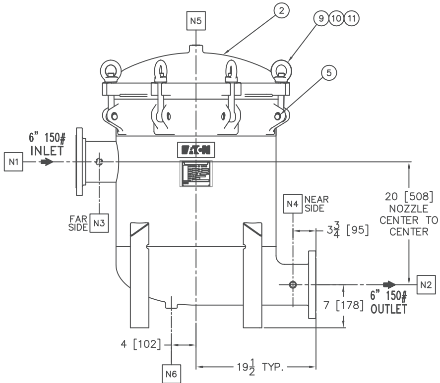
NOZZLE SCHEDULE
