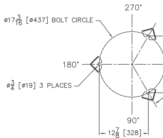
SECTION B-B MOUNTING PLAN
