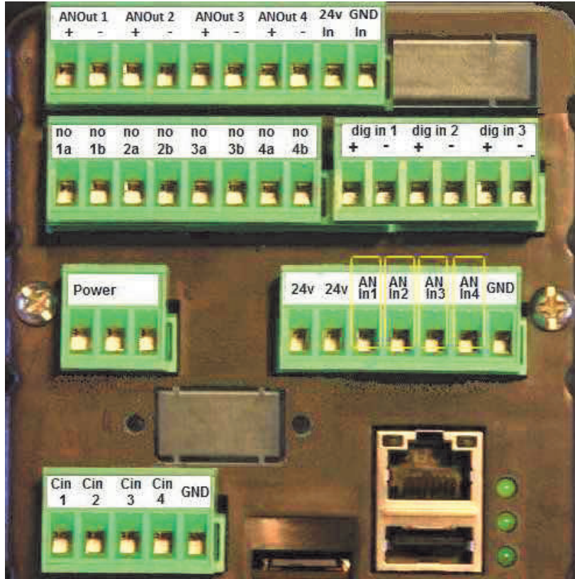
Figure 7-4 - During set-up of an analog probe to a 2300 with an analog output card, the analog output connector (on top) appears
