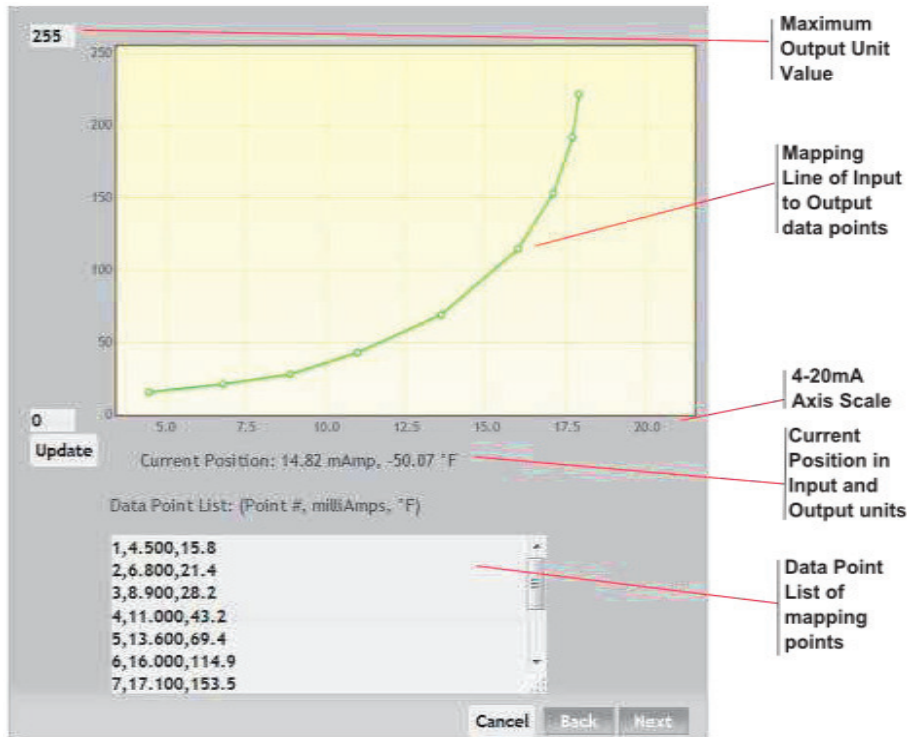
Figure 6-6 - Non-linear scaling window One must enter the calibration points manually into the bottom text box. This example shows a true non-linear scaling though this "non-linear" scaling can also be done for a linear output sensor.
