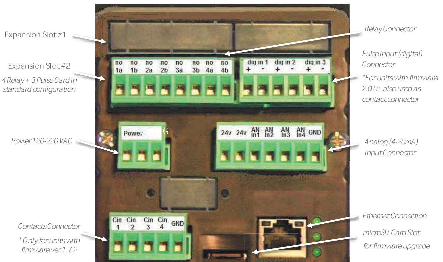
Figure 2-2 - 2300 Controller in standard configuration. Back panel view
