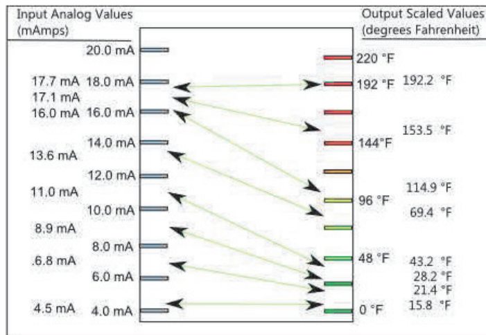
Figure 6-5 - Example of non-linear scaling. The 4-20 mA output of a temperature sensor is non-linear with temperature. To construct a non-linear scaling/calibration curve:
